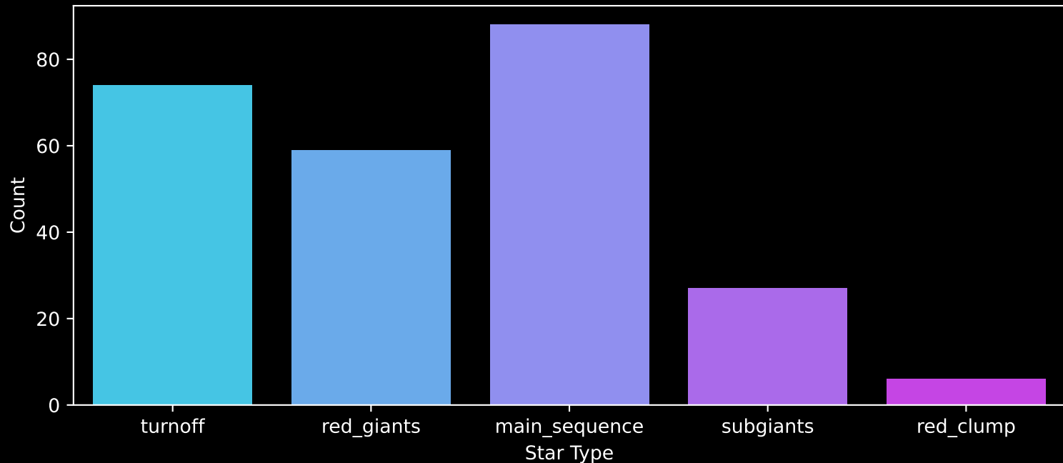
GALAH DR4 Field: [2845] Count plot of Star Type
