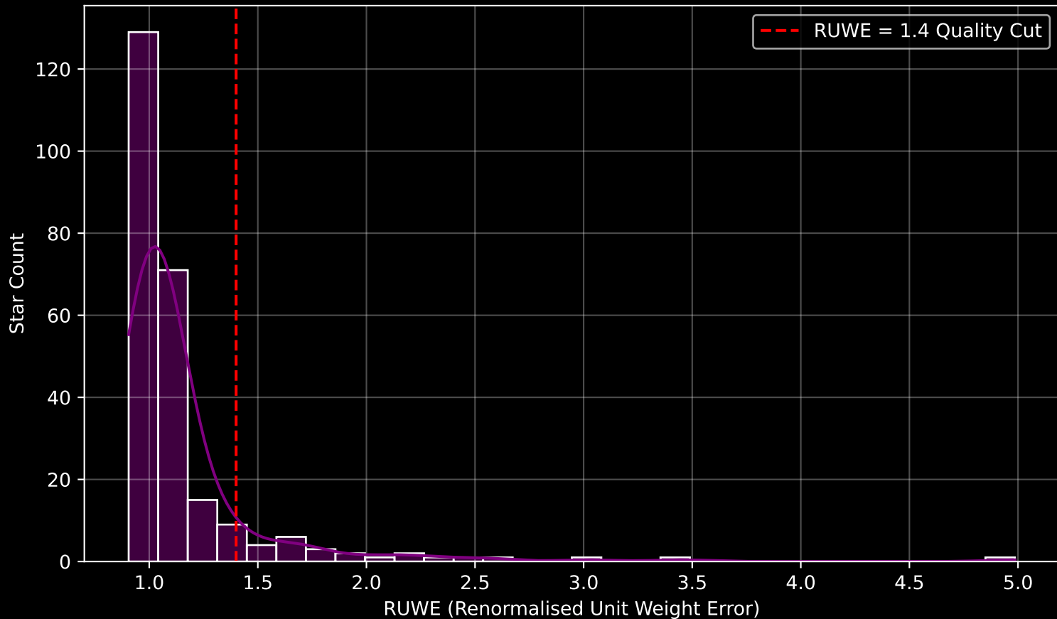
GALAH DR4 Field [2845] RUWE Distribution (n= 248)
